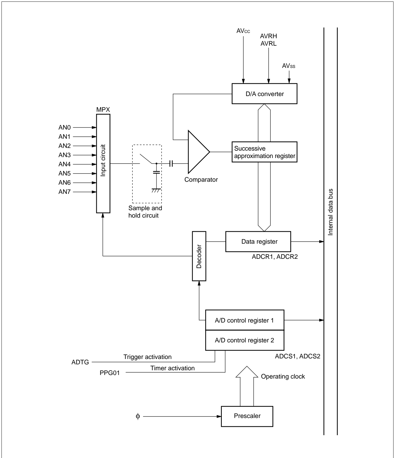
(2) Block Diagram
